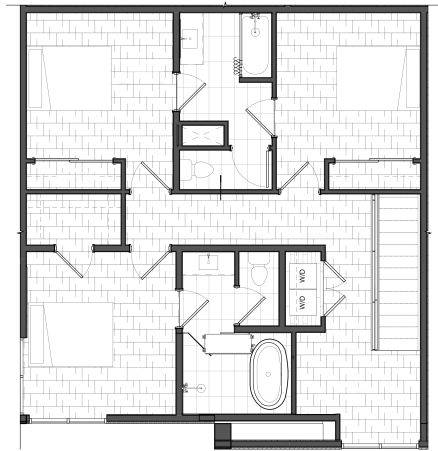
LEVEL ONE
